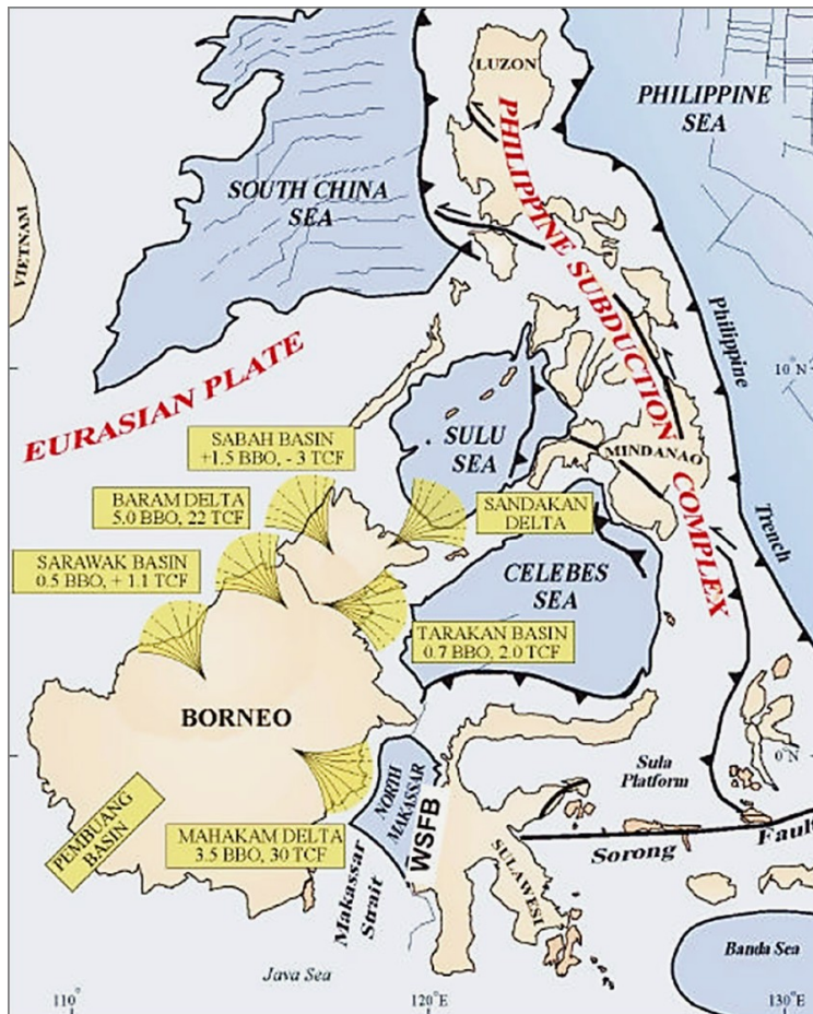
Figure IV.1.14. Diagrammatic map showing locations of major present-day delta systems around Borneo (Baillie et al. 2004, after Graves and Swaeger, 1997).
