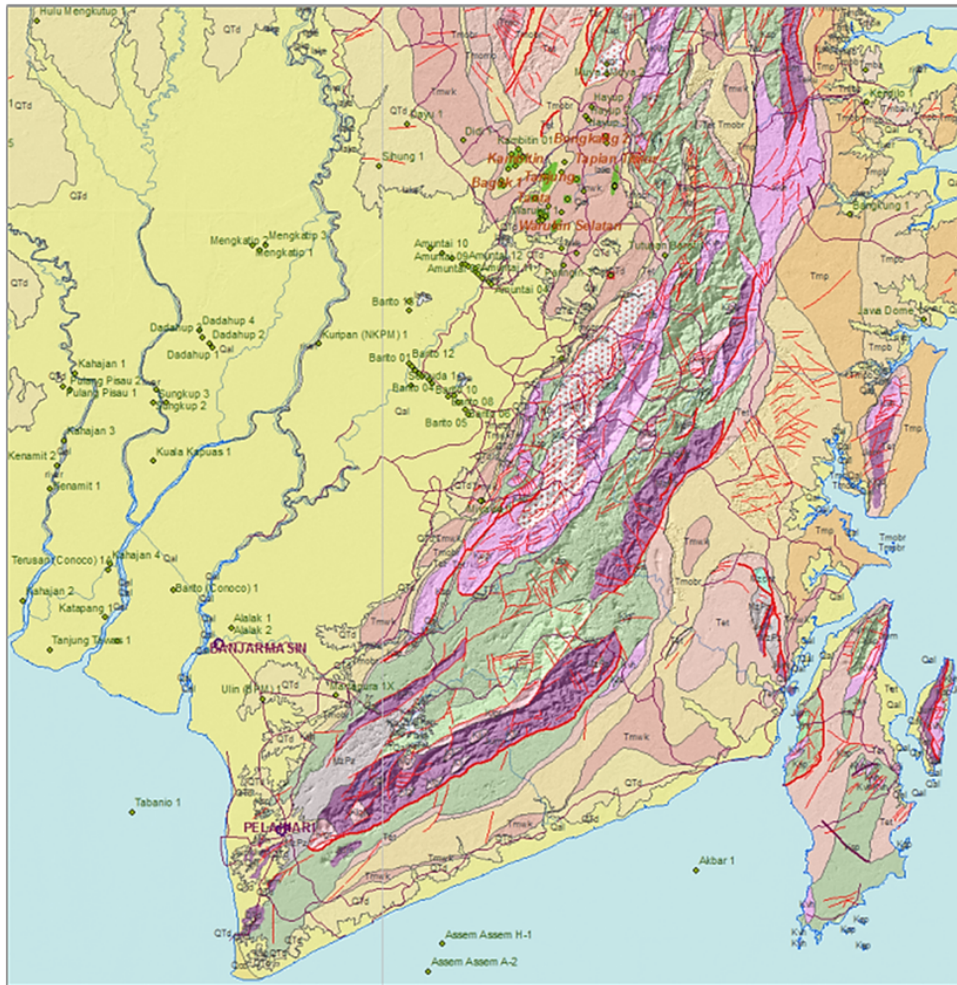
Figure IV.1.7. Meratus Mountains: a mid-Cretaceous collision complex with ophiolites, metamorphics and Late Cretaceous arc volcanics
