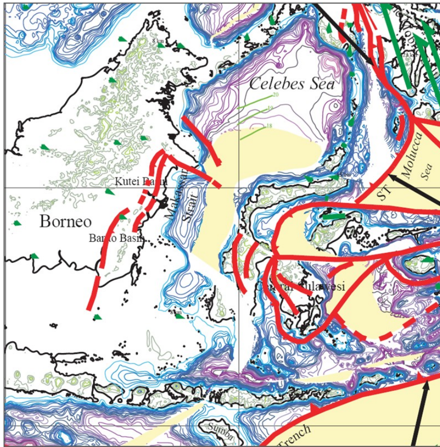
Figure IV.4.7. Plate position restoration of Sulawesi area at 10 Ma (Late Miocene) from 'backtracking' present-day GPS plate motions (Pubellier et al. 2005; DOTSEA project), suggesting the North Makassar Straits basin was twice the width of today. Yellow = areas of consumed (oceanic?) crust.
