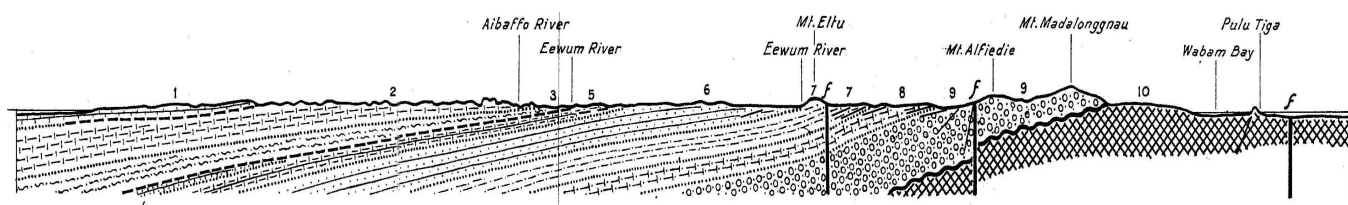
Figure VIII.10. N-S cross-section across N-dipping Triassic- Tertiary sediments of C Misool island (Roggeveen 1939 in Van Bemmelen, 1949)
