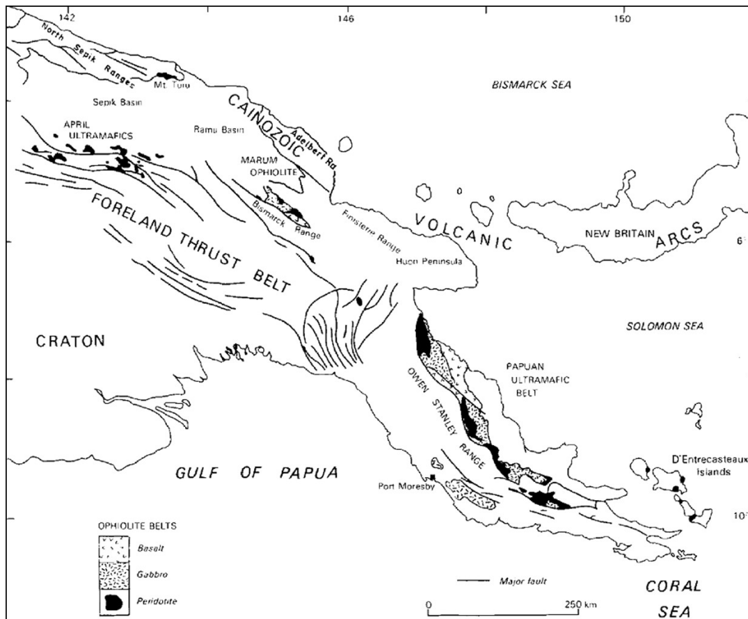
Figure VIII.17. Major ophiolite complexes of Papua New Guinea (Davies and Jaques, 1984)
