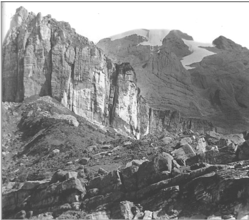
Figure VIII.3. Historic photo at ~4000m elevation of the ~4700m high, snow-covered peak of Mt. Wilhelm/Trikora (Hubrecht, Third South New Guinea Expedition 1912/1913). Showing a ridge (Upper Cretaceous?) bedded sandstone overlain by massive Cenozoic New Guinea Limestone.
