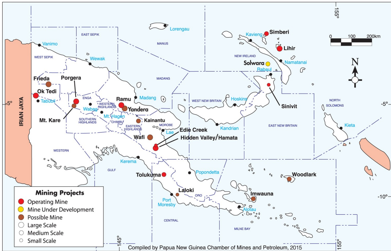
Figure VIII.21 . Map of main mining operations in Papua New Guinea.
