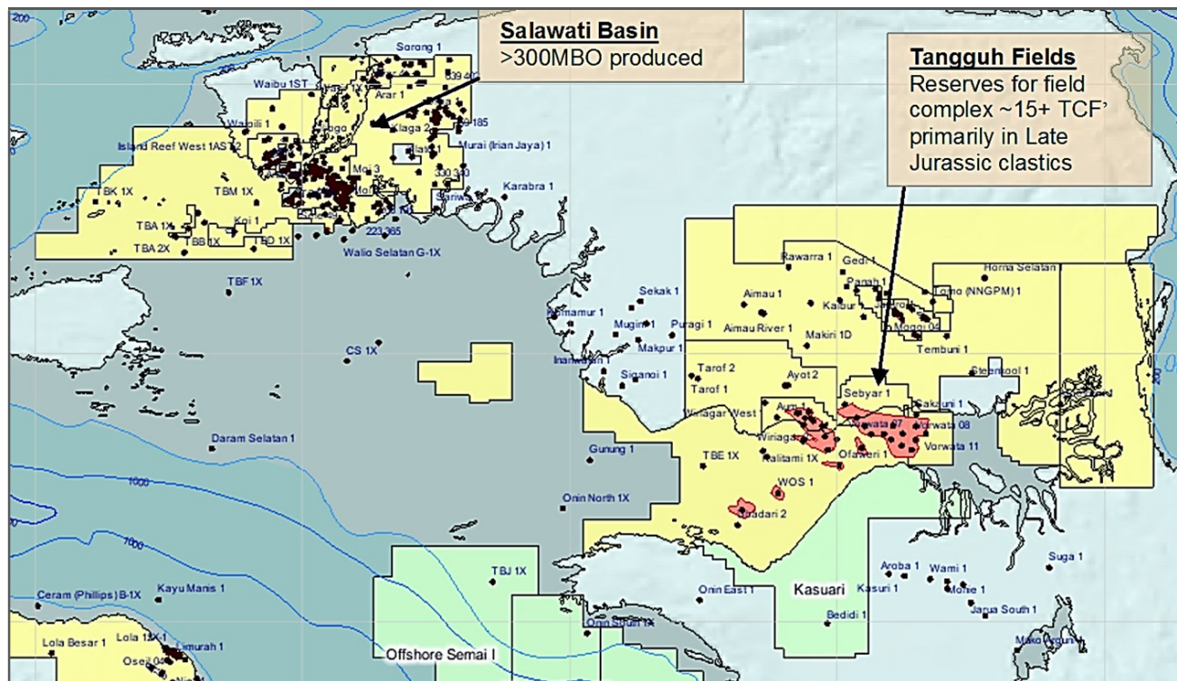
Figure VIII.6. Map of Birds Head- Bintuni Bay region, with well locations and large gas fields in Bintuni Bay (red) and small oil fields in the Salawati basin (basemap from IHS Energy, 2007).
