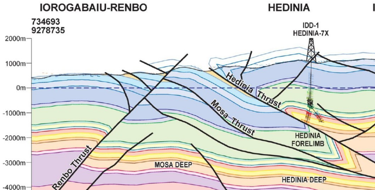
Figure VIII.20. Cross section of Iagafu- Hedinia field in frontal fold of PNG Central foldbelt (Hill et al. 2012)..
