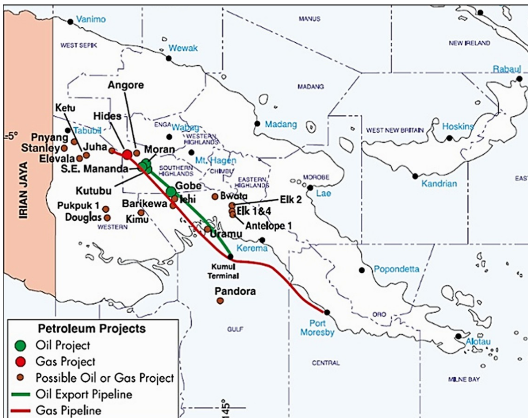
Figure VIII.19. Location map of main oil and gas fields of PNG (PNG Chamber of Mines and Petroleum).
