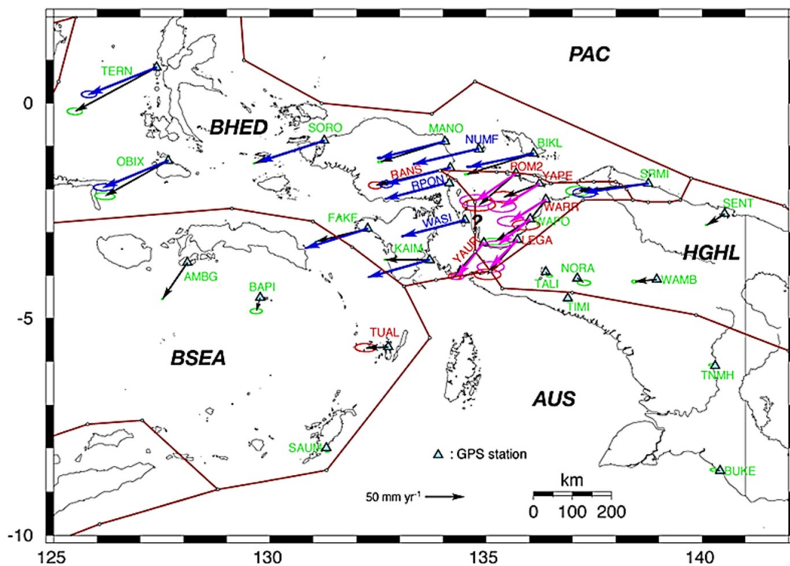
Figure VIII.5. Present-day GPS motions show Birds Head as part of a separate plate (BHED) that is very rapidly moving to the WSW relative to South New Guinea- North Australia (Tikku 2008).
