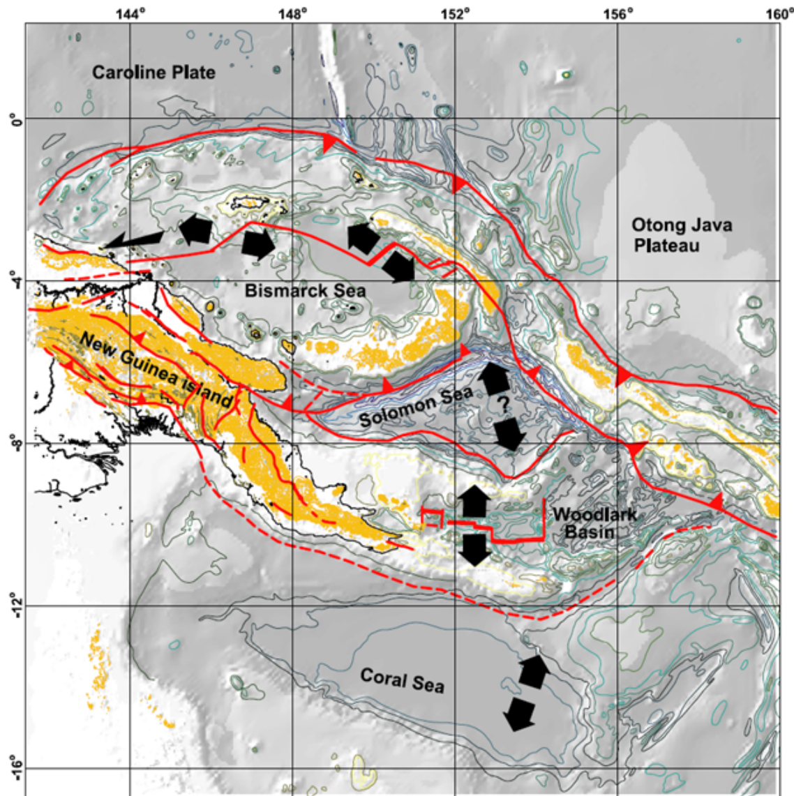
Figure VIII.25. Oceanic marginal basins developed NE and SE of Papua New Guinea main island, in zone of oblique convergence between the Australian and Pacific plates is now taken up at the New Guinea Trench and the Bismarck Sea spreading center(Manus Basin?) (Pubellier et al. 2004).
