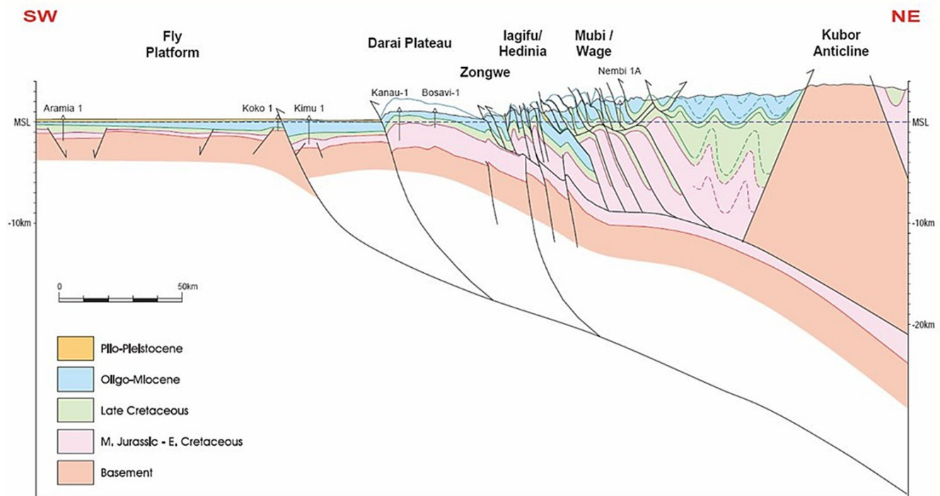
Figure VIII.15. Regional SW-NE cross-section across the Central Range of PNG (Oil Search, 2015, online).
