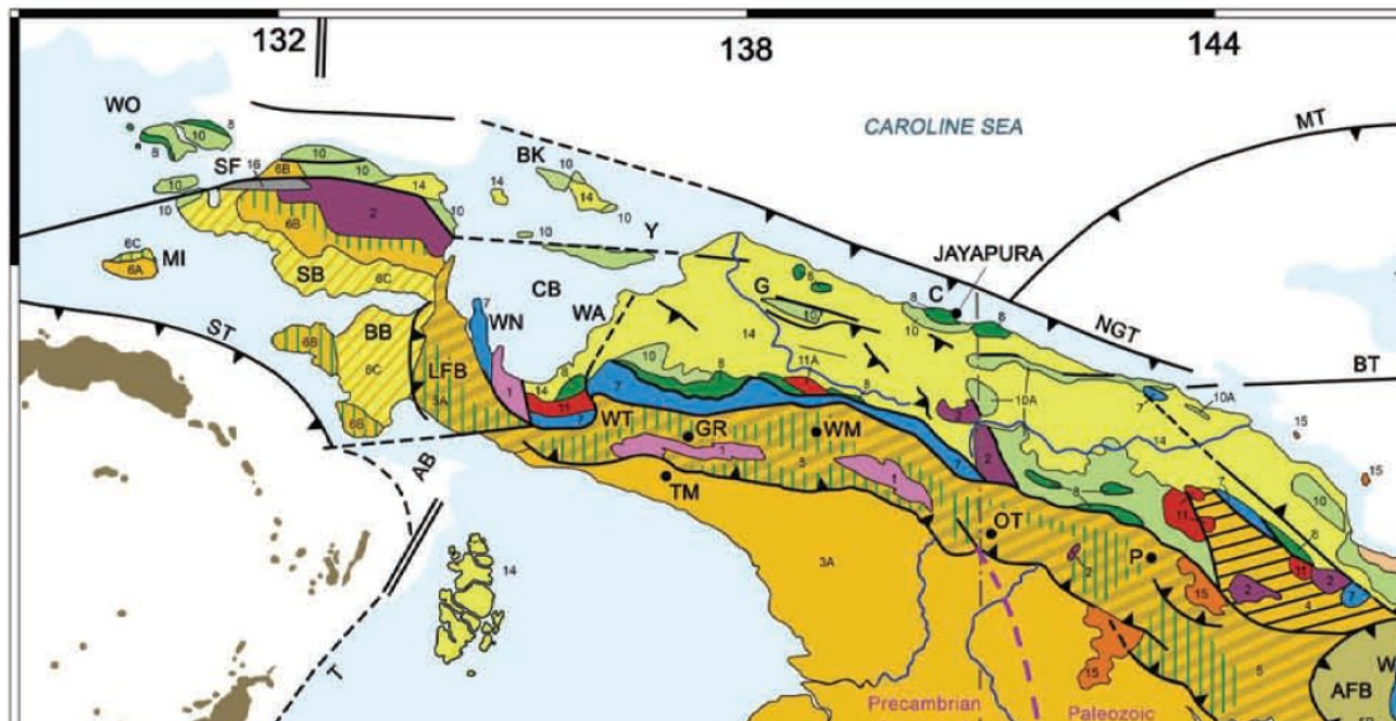
Figure VIII.2. Geological map of the New Guinea region (Davies 2012)
