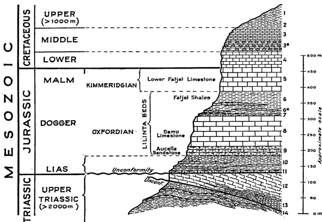
Figure VIII.11. Diagrammatic Mesozoic stratigraphy of Misool islands (Weber 1930, in Van Bemmelen, 1949)
