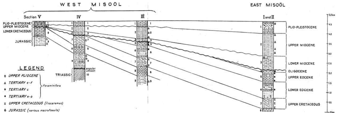
Figure VIII.12. W-E stratigraphic cross-section across Misool, showing 'mid-Oligocene' unconformity, most pronounced in West Misool (Roggeveen 1939 in Van Bemmelen, 1949).
