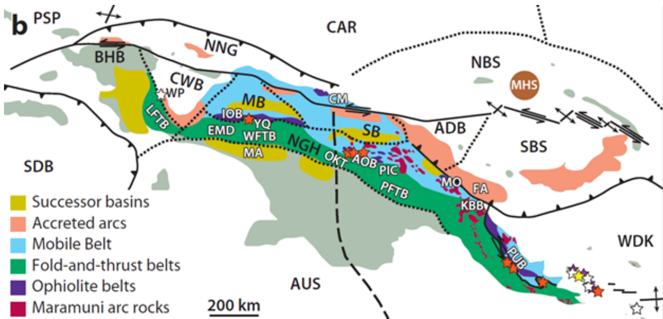
Figure VIII.1. Main tectonic elements of the New Guinea region (Baldwin et al. 2012)
