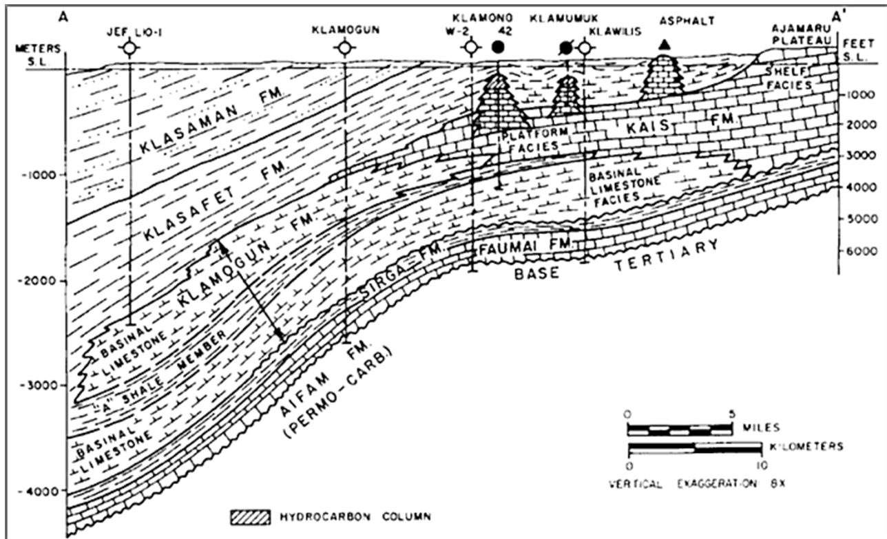
Figure VIII.7. Schematic W-E cross section through the Salawati Neogene foreland basin, showing backstepping Late Miocene Kais carbonate platform and reefal buildups (Vincelette & Soeparjadi 1976).
