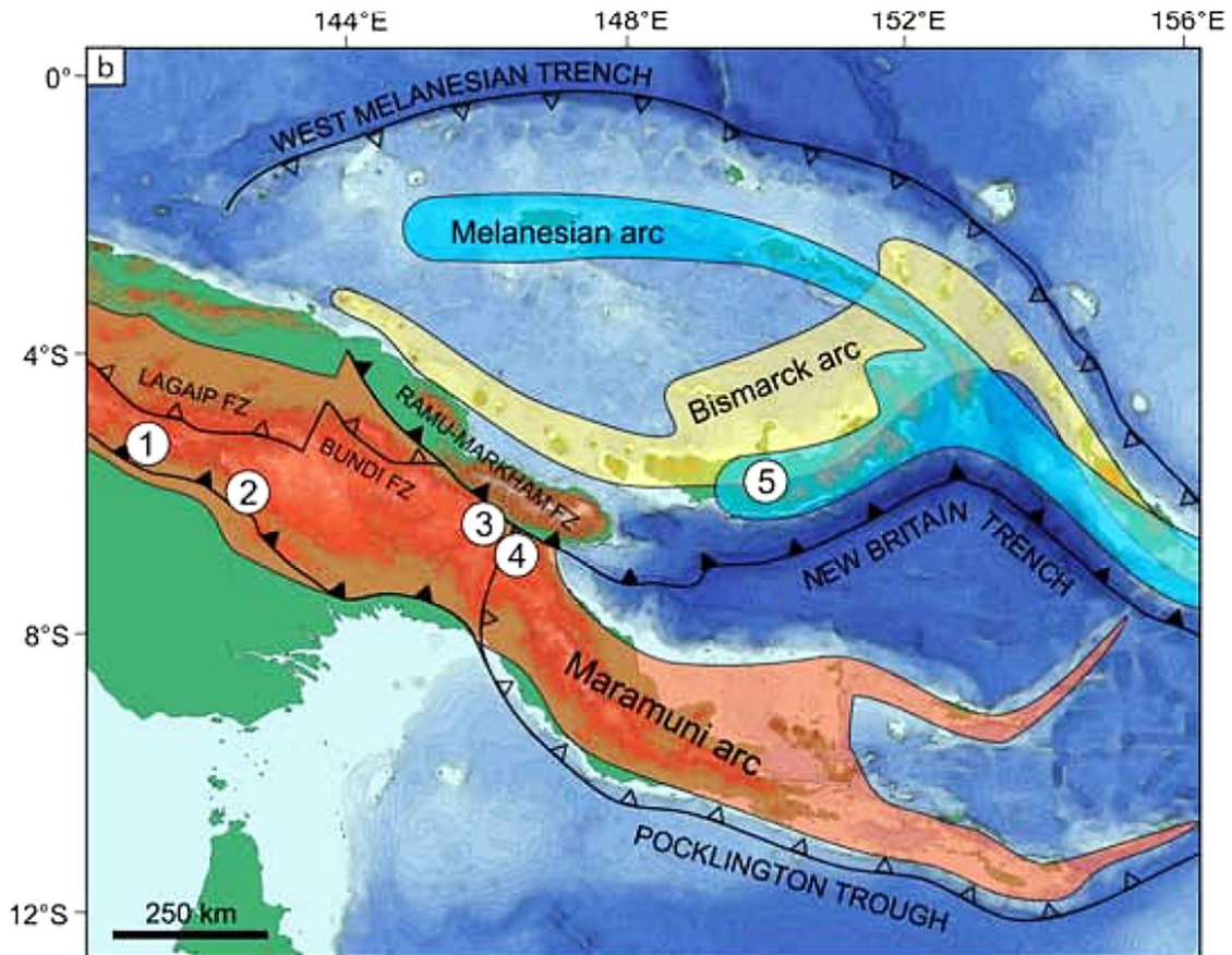
Figure VIII.22. Neogene- Recent magmatic arcs of Papua New Guinea, with corresponding subduction zones (Holm et al. 2013).
