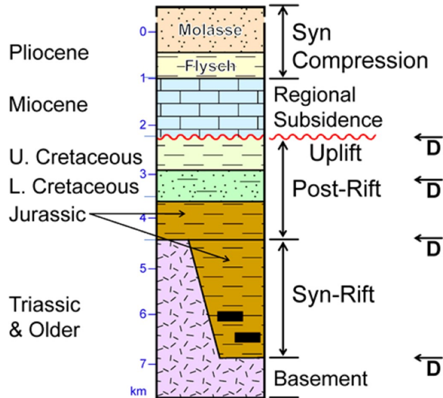
Figure VIII.16. Diagrammatic stratigraphy of Mesozoic- Tertiary of Papua- New Guinea foldbelt, with approximate thicknesses. (Juha field; Hanani et al. (2016). Mesozoic rift- passive margin sequence, Upper Cretaceous uplift event, Plio-Pleistocene syn-compressional flysch and molasse. D= detachment surfaces.
