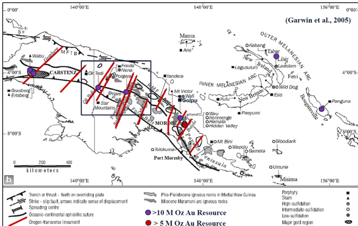
Figure VIII.8. Principal copper-gold deposits of New Guinea (Garwin et al. 2005). Major porphyry copper-gold systems are tied to intersections of the magmatic belt and steep transverse faults.
