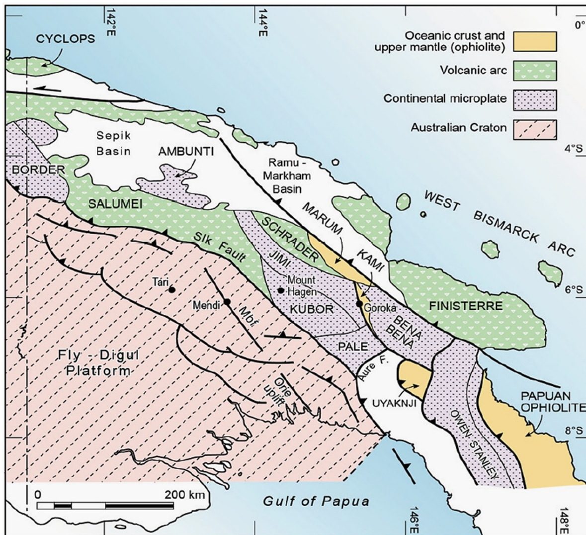
Figure VIII.13. Tectonostratigraphic terranes of Papua New Guinea main island. Sik Fault= Stolle-Lagaip-Kaugel fault that separates autochthonous Australian plate in South from allochthonous accreted terranes in North (Glen et al. 2016, after Davies et al. 1996)
